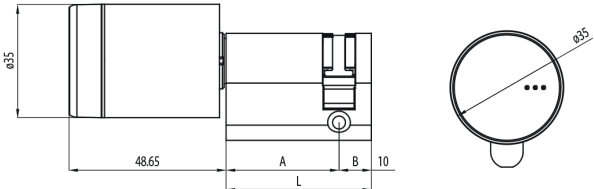
Euro profile single knob cylinder
