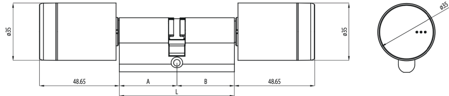
Euro profile double knob cylinder
